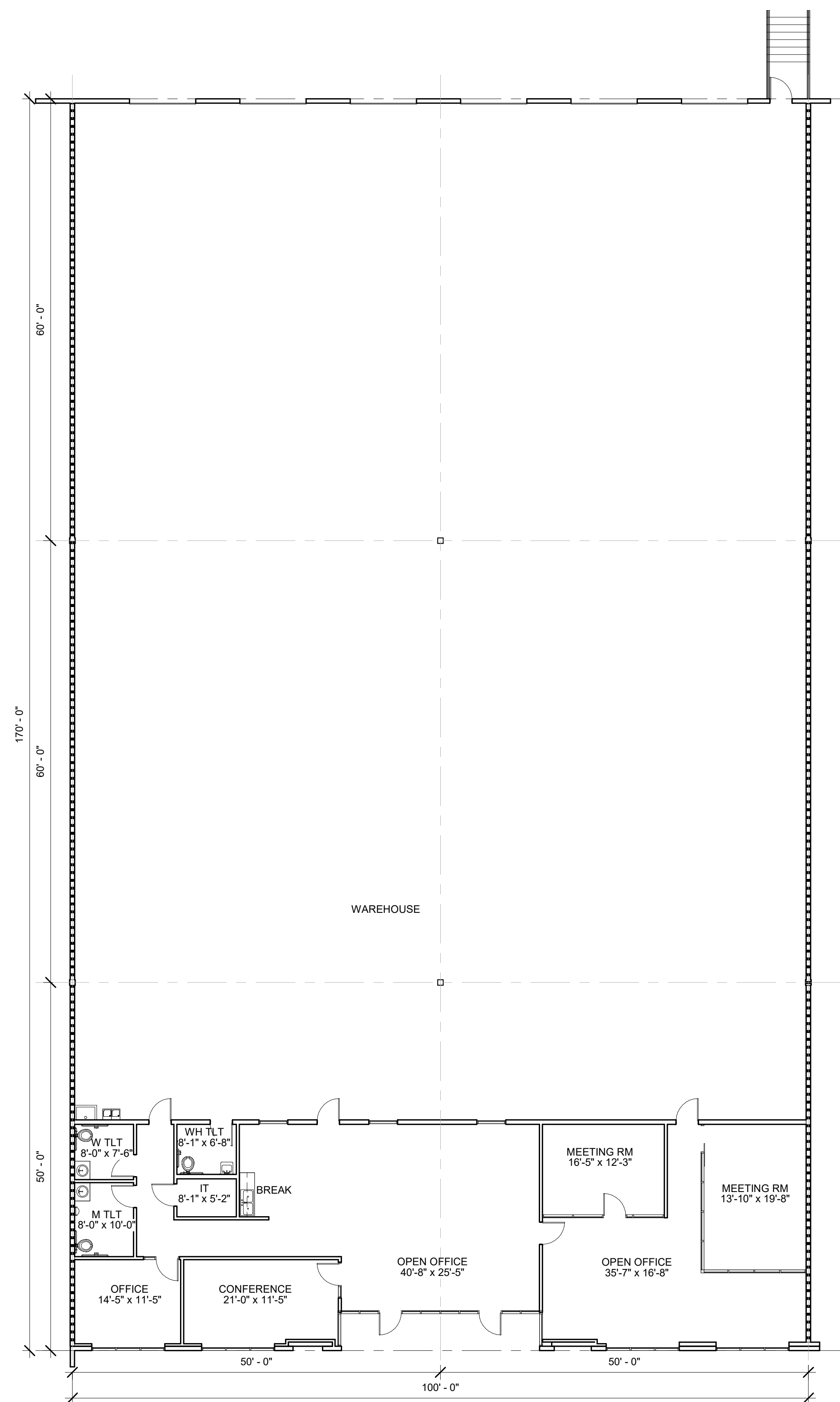
① As-Built Floor Plan 3/32" = 1'-0"
