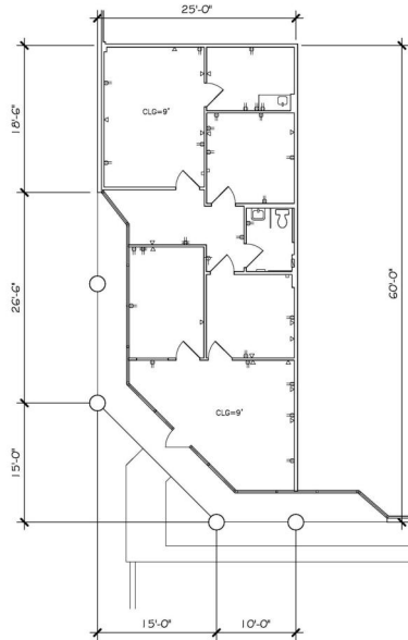
1,388 SQ.FT. EXISTING PLAN 10-9-24 CLG = CEILING HEIGHT 1" = 10' WEST LOOP CENTRE 5419 BANDERA ROAD #703 SAN ANTONIO, TX. 78238
