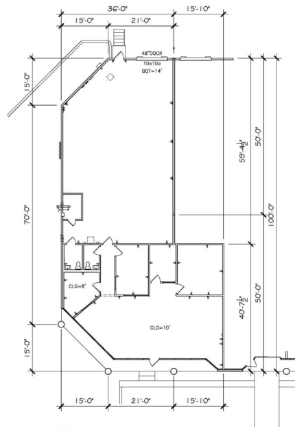
OFFICE AREA = 1,792sf 4,025 SQ.FT. EXISTING PLAN 9-26-24 CLG = CEILING HEIGHT BOT = BOTTOM OF TRUSS 1/16" = 1'-0" WEST LOOP CENTRE 5415 BANDERA ROAD #501 SAN ANTONIO, TX. 78238
