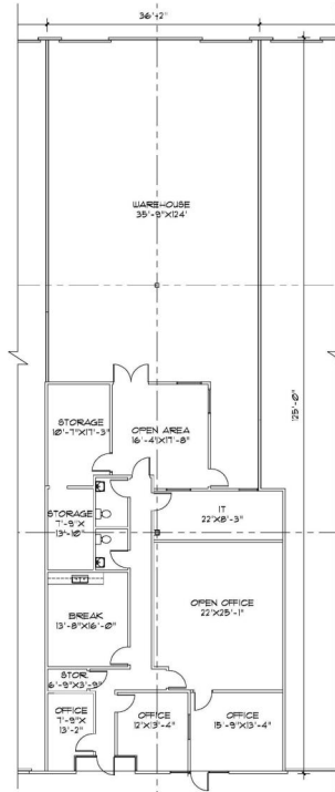
LEASE PLAN SCALE: 3/32"=1'-0" NOTE: ALL DIMENSIONS ARE APPROXIMATE AND ALL INFORMATION IS OF GENERAL NATURE
